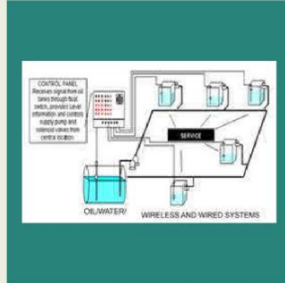
Water Level Indicator And Controller For Multiple Tanks
